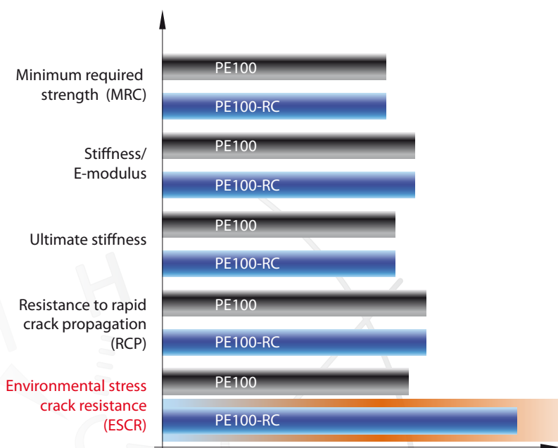
Comparison of PE100-RC material with PE100 material
