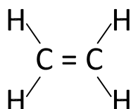
Ethylene Molecule
