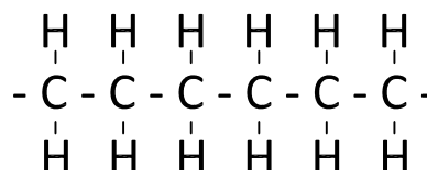
Polyethylene Molecule
